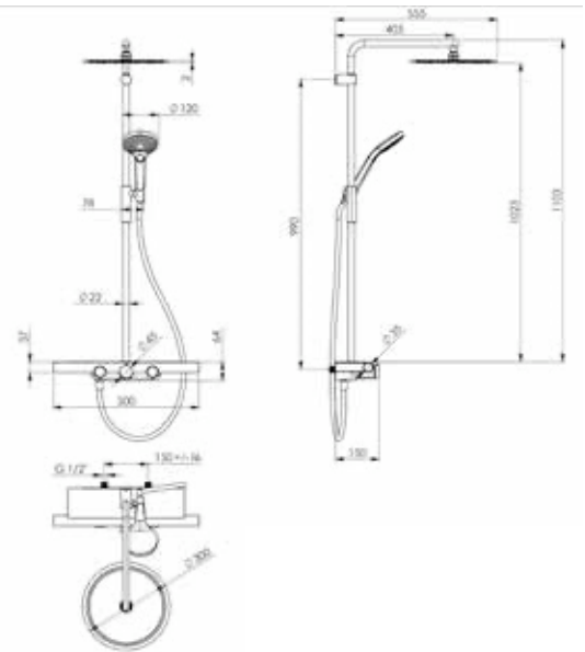
PM10200/MB-MG With Matte Brushed Gold metal handles
