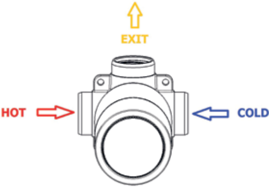
Flow opening/closing
